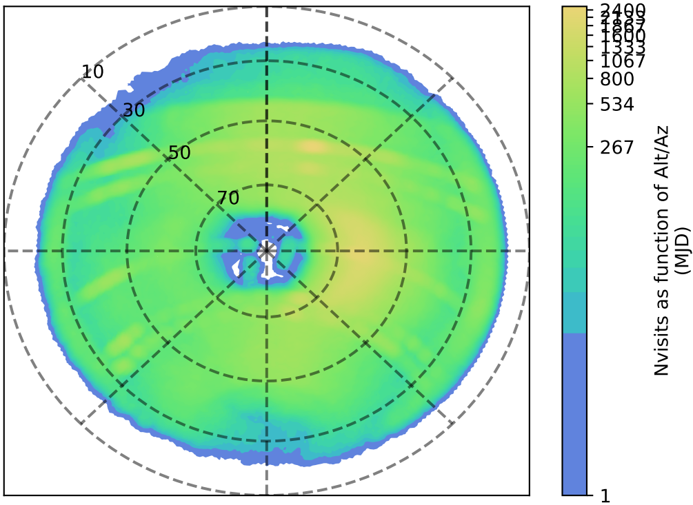
too_elab_2yr_r32_d3_ugrizy_v3.4_10yrs z: Nvisits as function of Alt/Az
