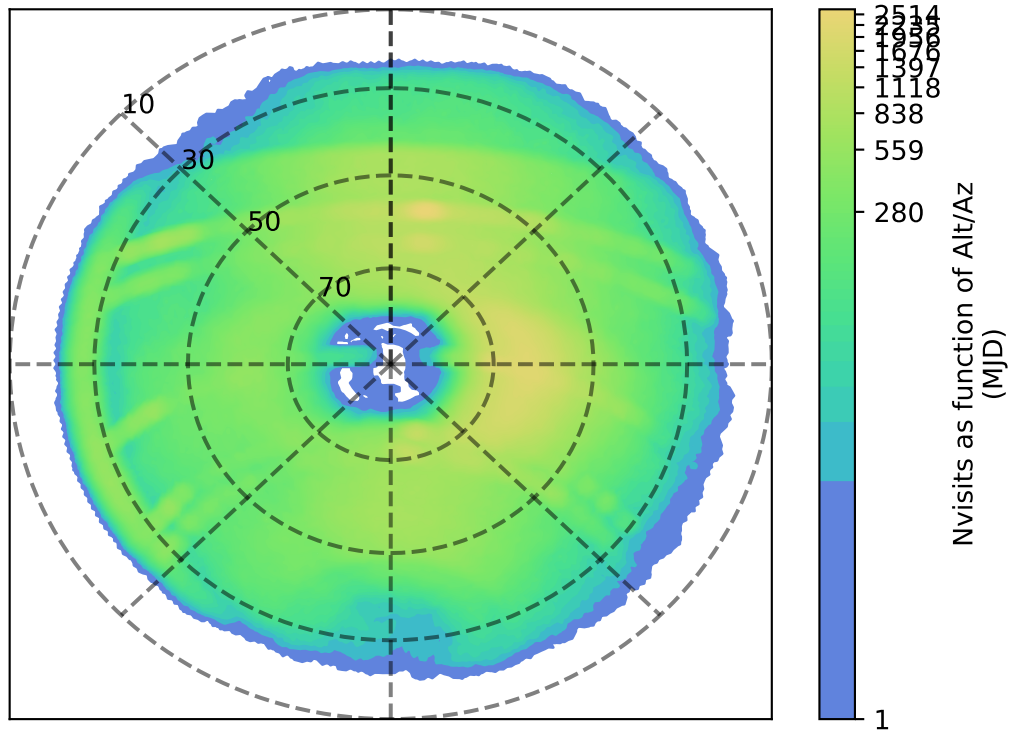
too_elab_2yr_r32_d3_ugrizy_v3.4_10yrs r: Nvisits as function of Alt/Az
