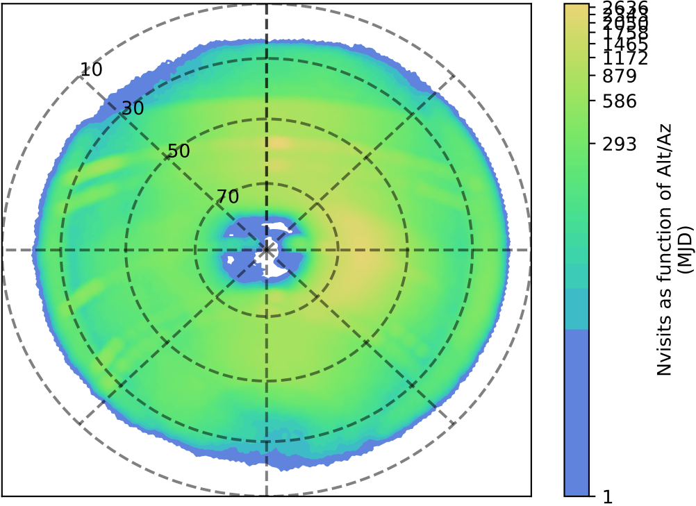
too_elab_2yr_r32_d3_ugrizy_v3.4_10yrs i: Nvisits as function of Alt/Az
