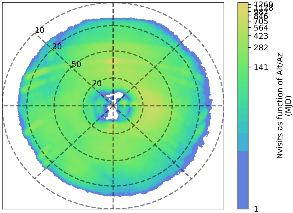
too_elab_2yr_r32_d3_ugrizy_v3.4_10yrs g: Nvisits as function of Alt/Az
