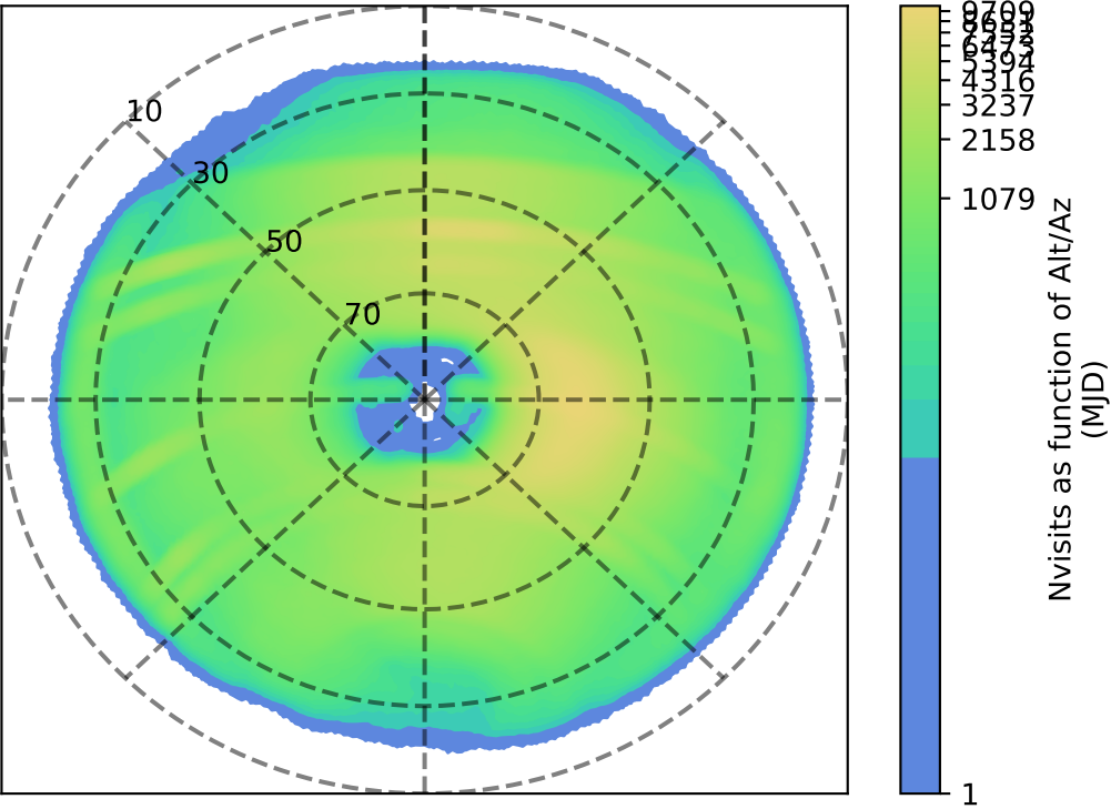
too_elab_2yr_r32_d3_ugrizy_v3.4_10yrs : Nvisits as function of Alt/Az
