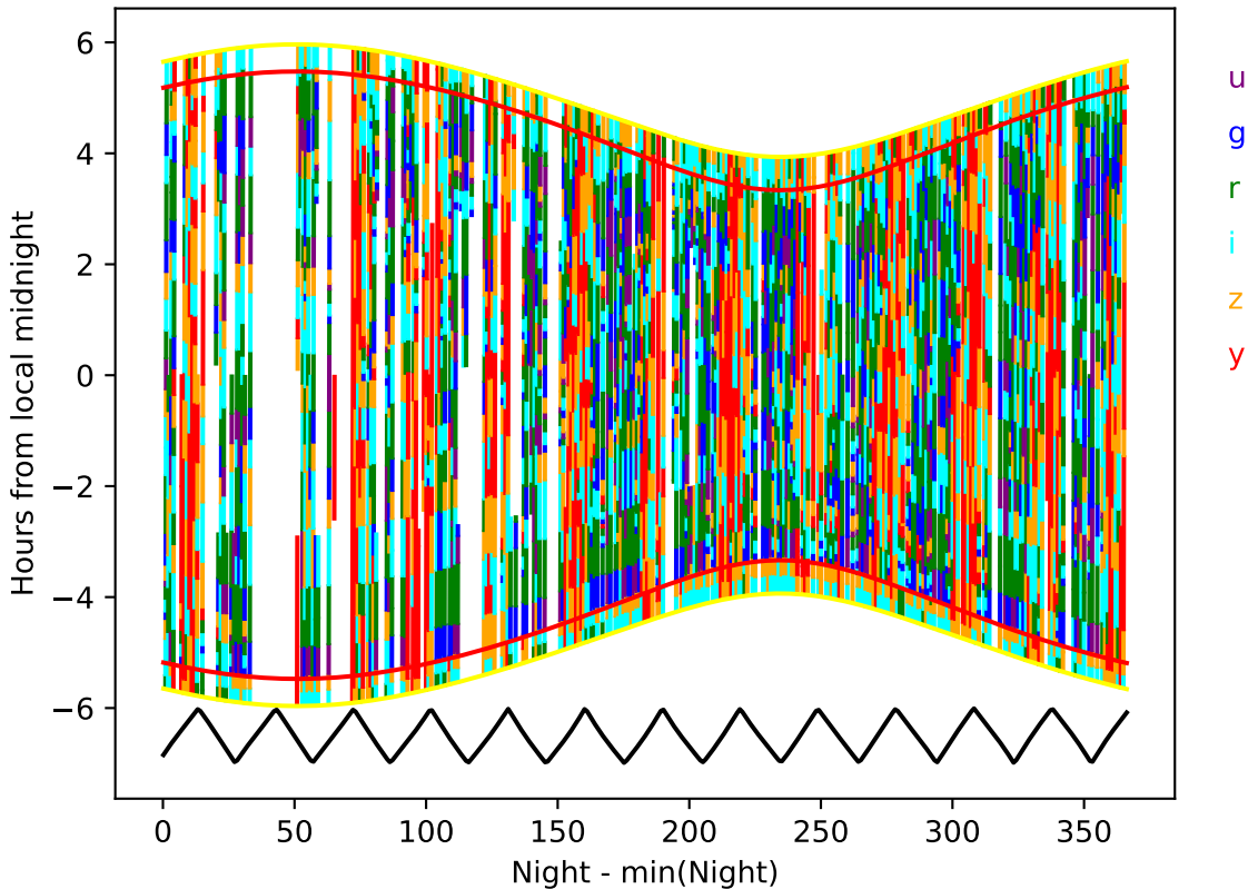
too_elab_2yr_r32_d3_ugrizy_v3.4_10yrs year 8-9: Hourglass
