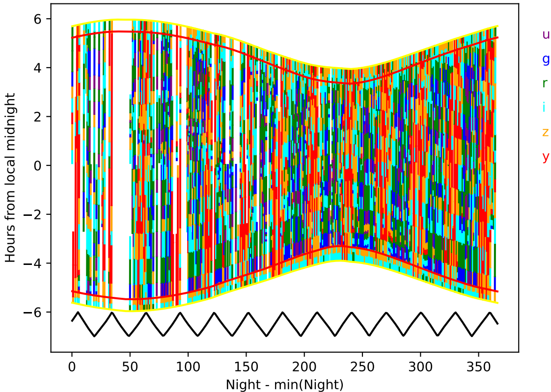
too_elab_2yr_r32_d3_ugrizy_v3.4_10yrs year 6-7: Hourglass
