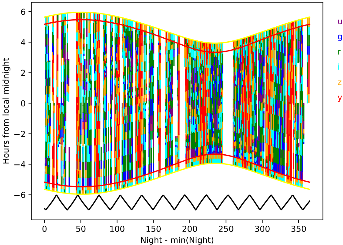
too_elab_2yr_r32_d3_ugrizy_v3.4_10yrs year 5-6: Hourglass
