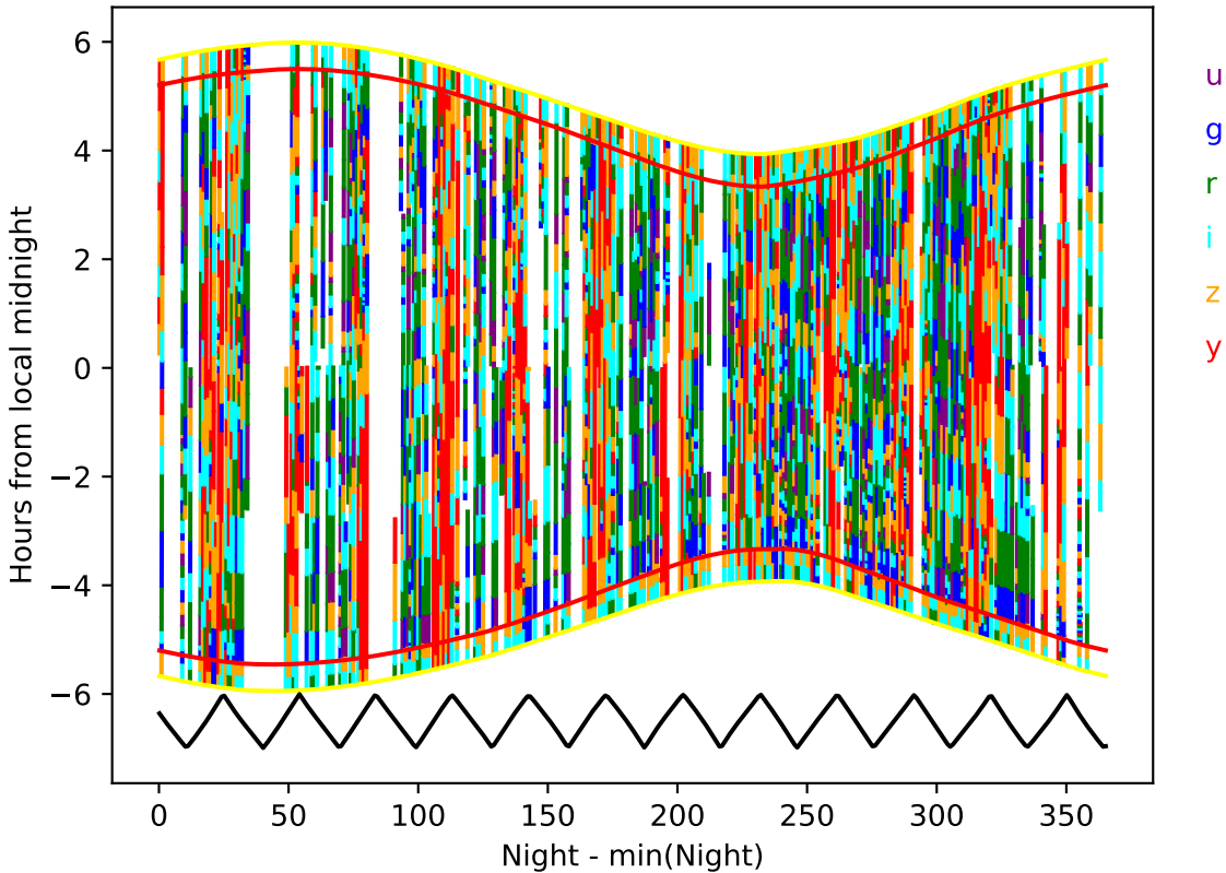
too_elab_2yr_r32_d3_ugrizy_v3.4_10yrs year 4-5: Hourglass
