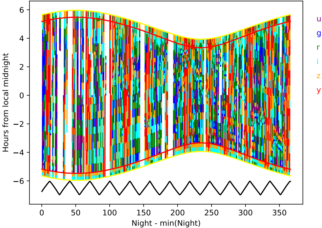
too_elab_2yr_r32_d3_ugrizy_v3.4_10yrs year 0-1: Hourglass
