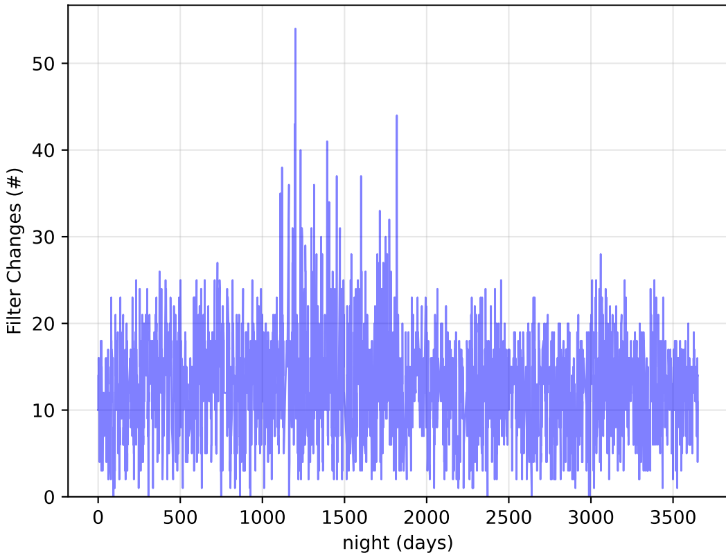
too_elab_2yr_r32_d3_ugrizy_v3.4_10yrs : Filter Changes
