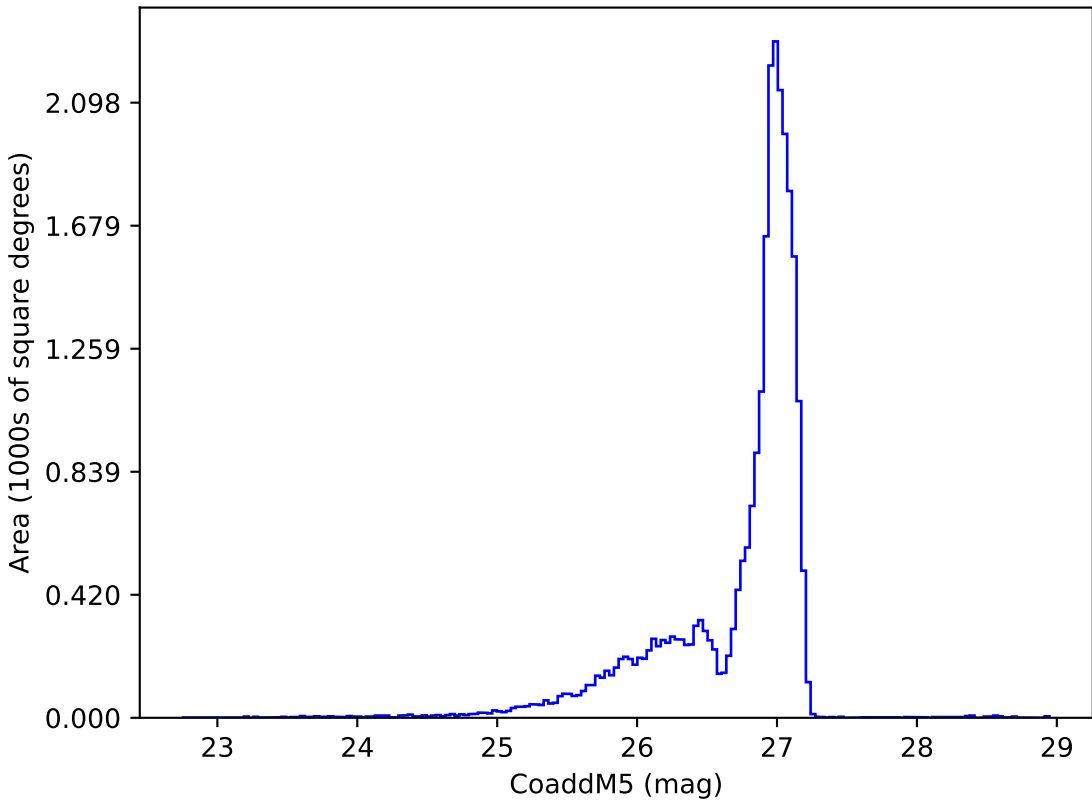
too_elab_2yr_r32_d3_ugrizy_v3.4_10yrs r: CoaddM5
