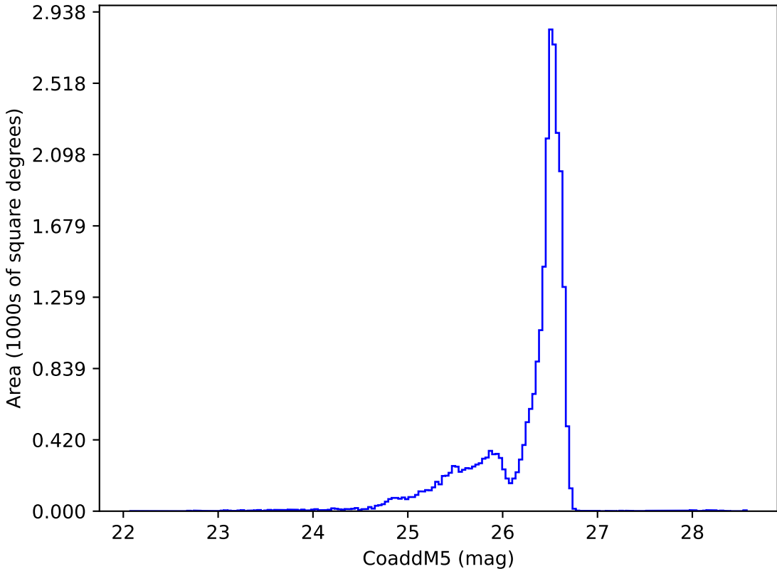
too_elab_2yr_r32_d3_ugrizy_v3.4_10yrs i: CoaddM5
