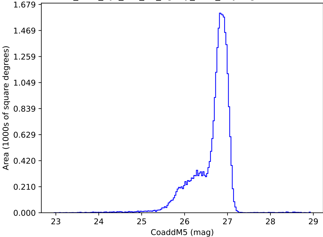
too_elab_2yr_r32_d3_ugrizy_v3.4_10yrs g: CoaddM5
