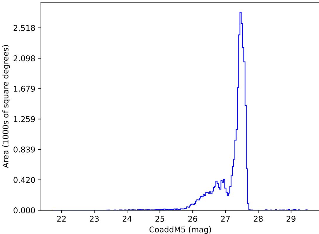
too_elab_2yr_r32_d3_ugrizy_v3.4_10yrs : CoaddM5
