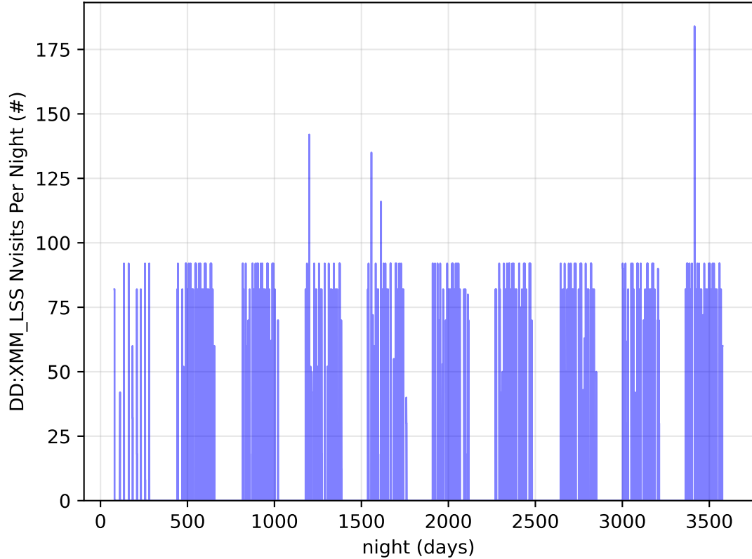
too_elab_2yr_r32_d3_ugrizy_v3.4_10yrs all bands: DD:XMM_LSS Nvisits Per Night
