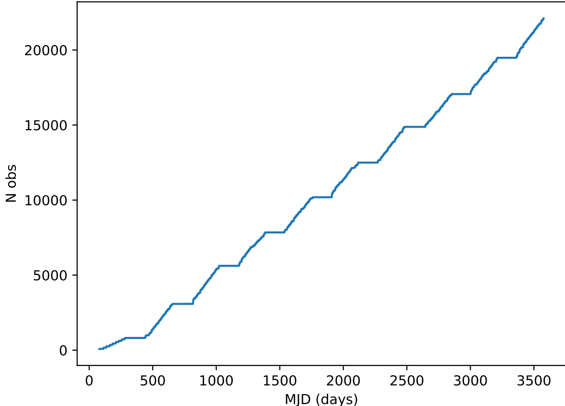
too_elab_2yr_r32_d3_ugrizy_v3.4_10yrs all bands: DD:XMM_LSS Cumulative NVisits
