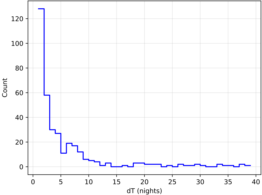
too_elab_2yr_r32_d3_ugrizy_v3.4_10yrs all bands: DD:WFD Delta Nights Histogram
