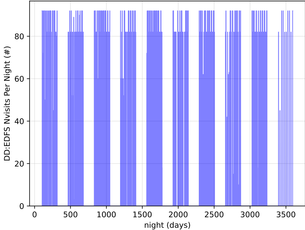
too_elab_2yr_r32_d3_ugrizy_v3.4_10yrs all bands: DD:EDFS Nvisits Per Night
