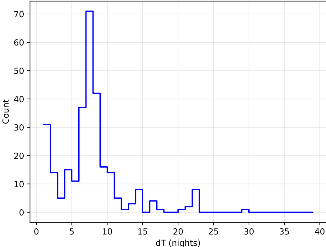
too_elab_2yr_r32_d3_ugrizy_v3.4_10yrs all bands: DD:EDFS Delta Nights Histogram
