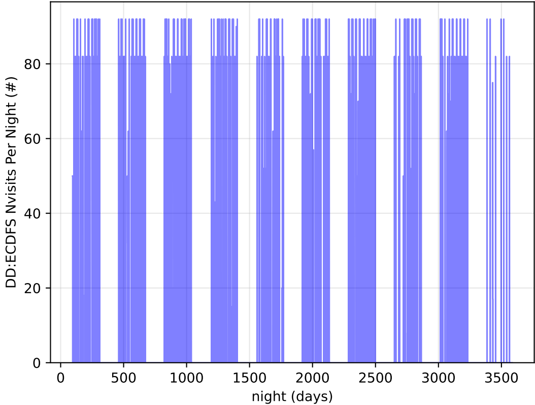
too_elab_2yr_r32_d3_ugrizy_v3.4_10yrs all bands: DD:ECDFS Nvisits Per Night
