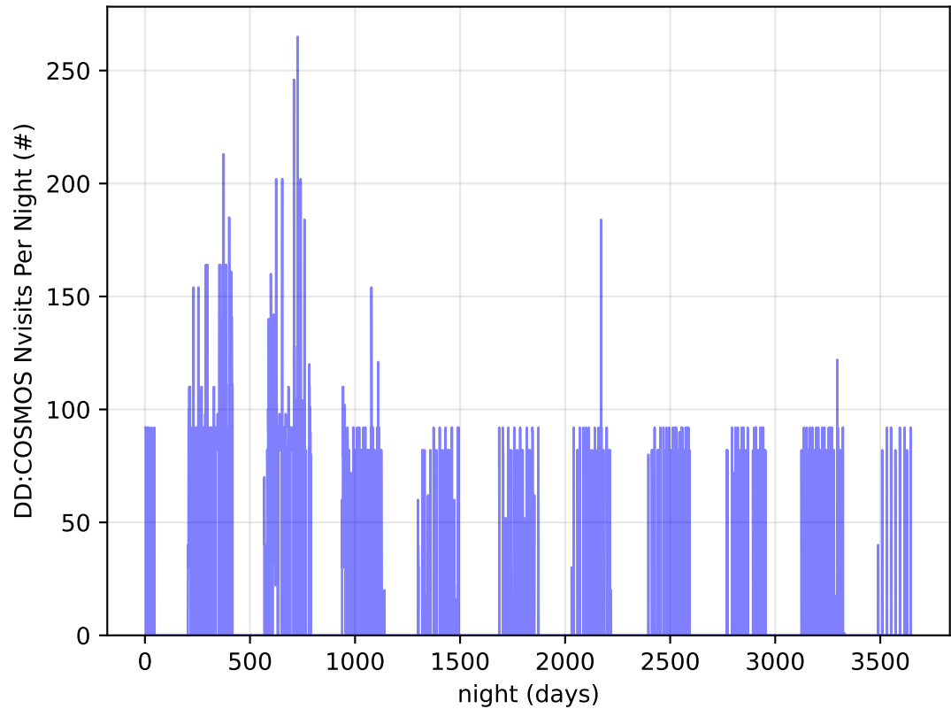
too_elab_2yr_r32_d3_ugrizy_v3.4_10yrs all bands: DD: COSMOS Nvisits Per Night
