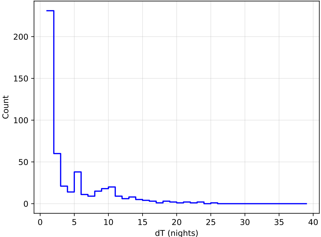
too_elab_2yr_r32_d3_ugrizy_v3.4_10yrs all bands: DD: COSMOS Delta Nights Histogram
