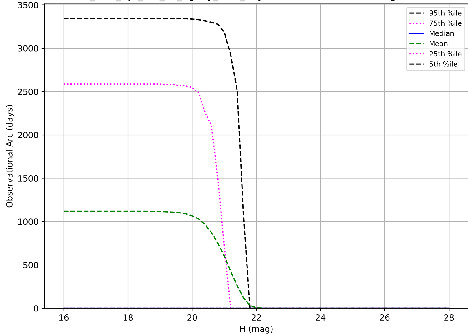
too_elab_2yr_r32_d2_ugrizy_v3.4_10yrs: Observational Arc Length Vatira
