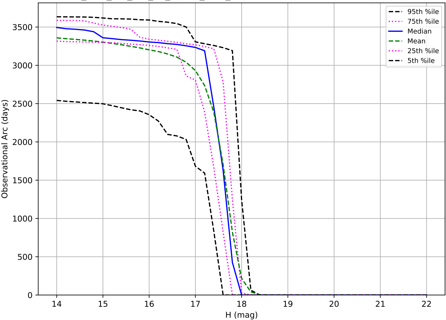
too_elab_2yr_r32_d2_ugrizy_v3.4_10yrs: Observational Arc Length Trojan
