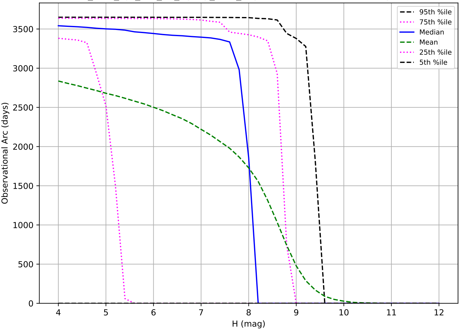
too_elab_2yr_r32_d2_ugrizy_v3.4_10yrs: Observational Arc Length TNO
