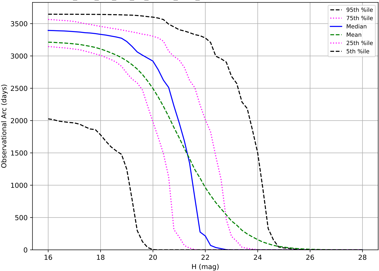
too_elab_2yr_r32_d2_ugrizy_v3.4_10yrs: Observational Arc Length PHA
