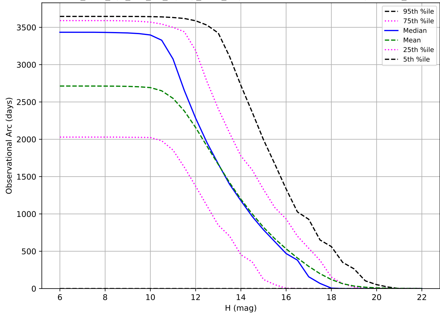
too_elab_2yr_r32_d2_ugrizy_v3.4_10yrs: Observational Arc Length OCC_r5
