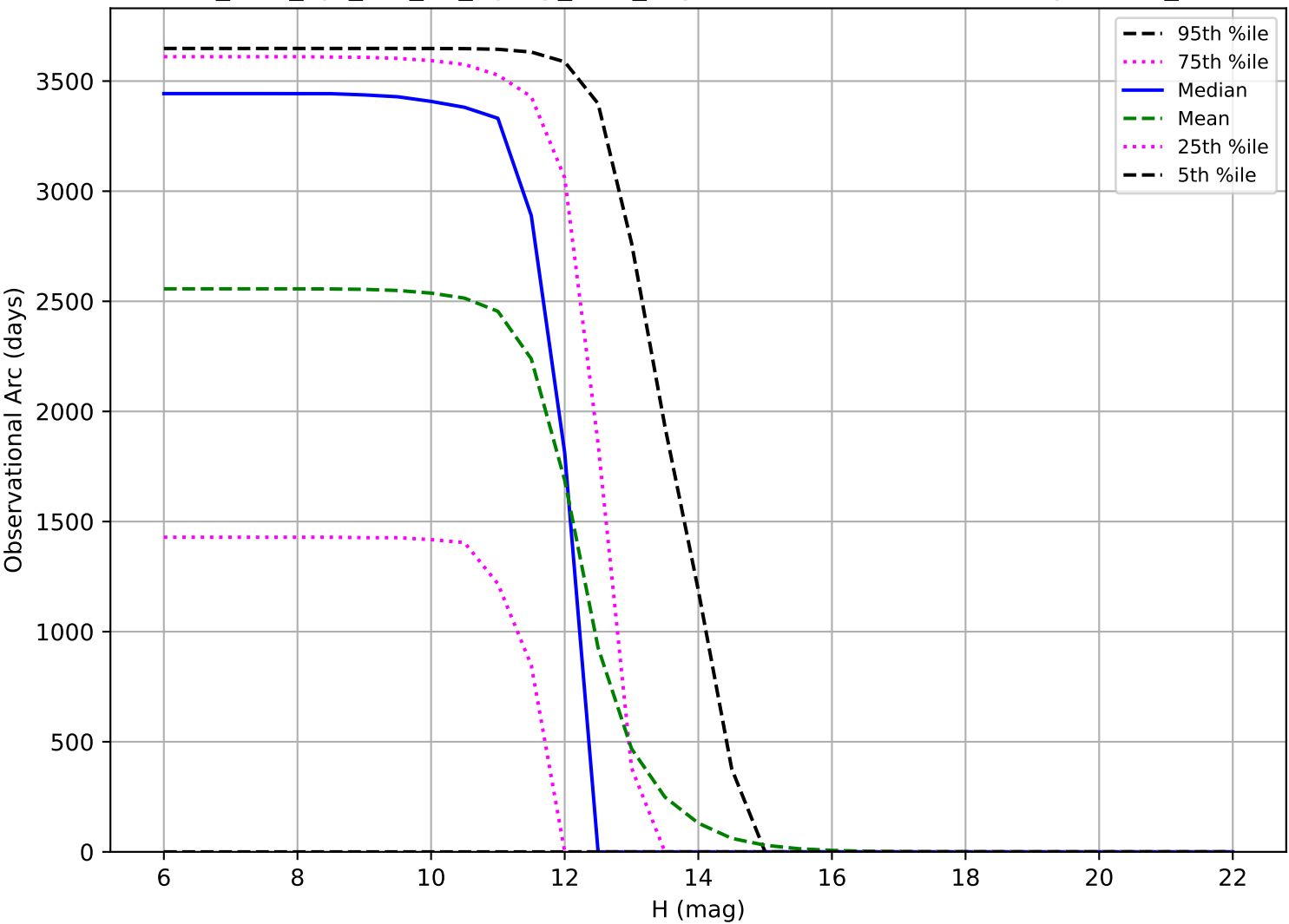
too_elab_2yr_r32_d2_ugrizy_v3.4_10yrs: Observational Arc Length OCC_r20
