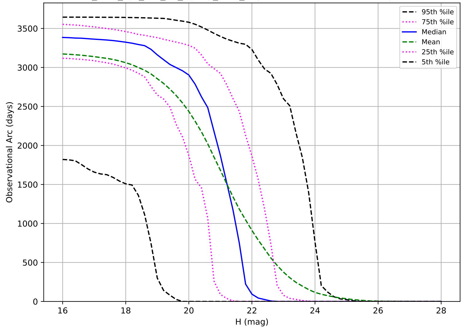
too_elab_2yr_r32_d2_ugrizy_v3.4_10yrs: Observational Arc Length NEO
