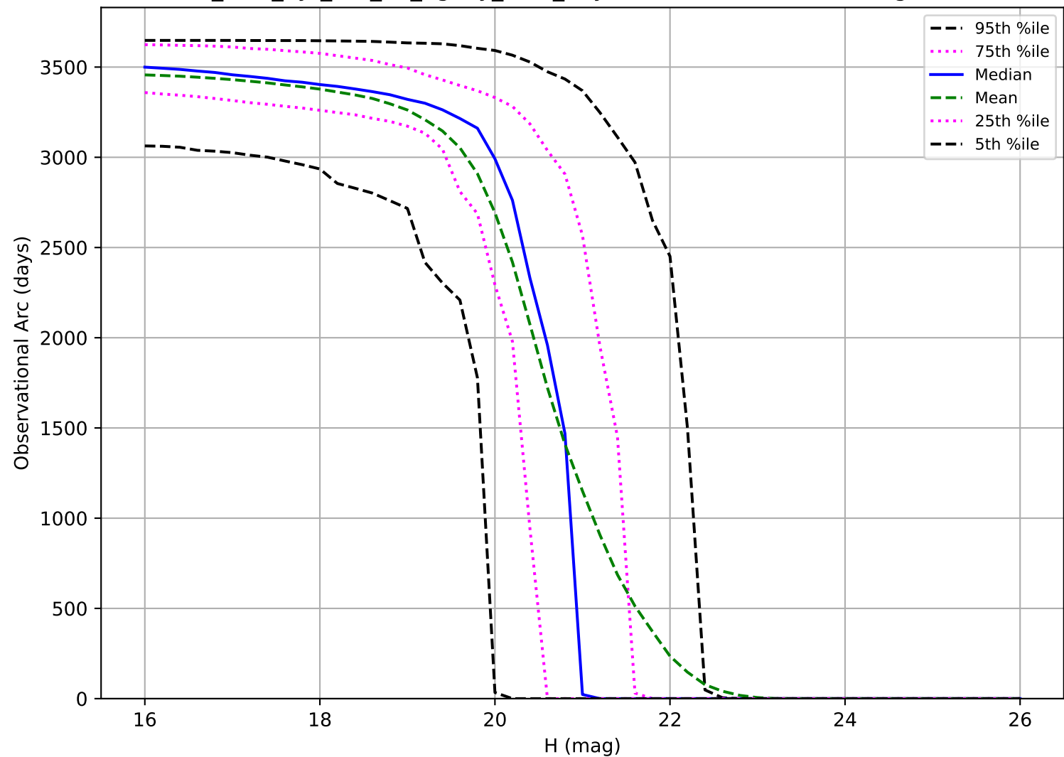
too_elab_2yr_r32_d2_ugrizy_v3.4_10yrs: Observational Arc Length MBA
