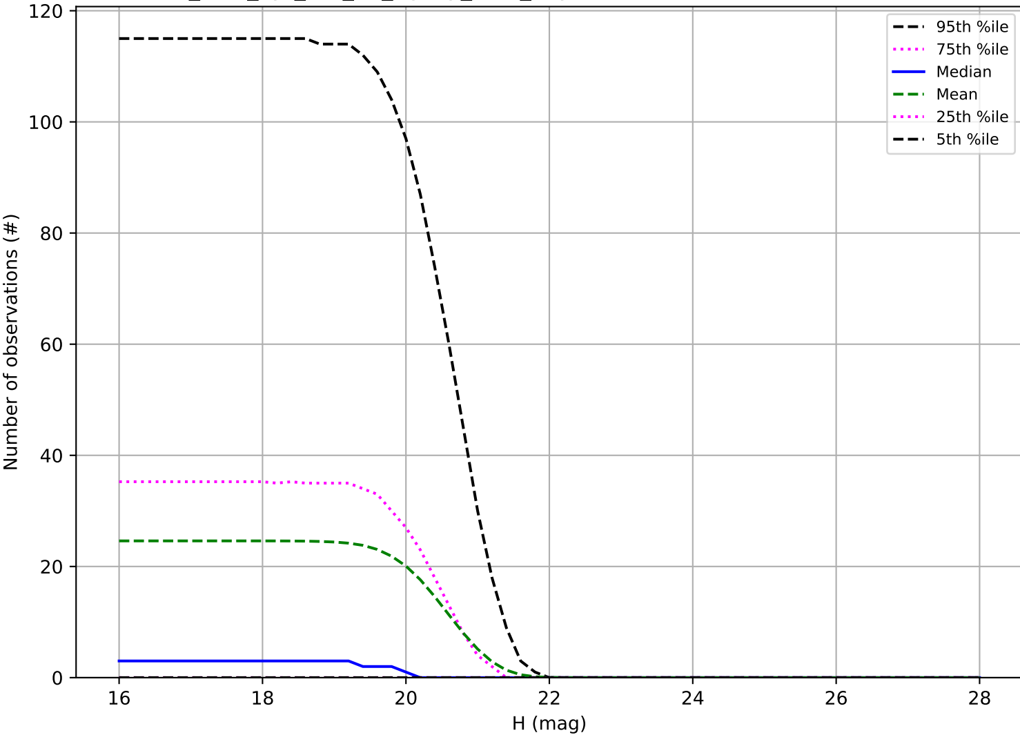
too_elab_2yr_r32_d2_ugrizy_v3.4_10yrs: Number of observations Vatira
