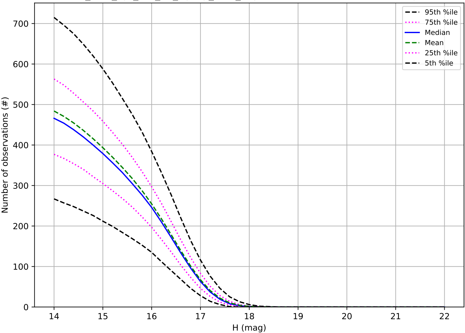
too_elab_2yr_r32_d2_ugrizy_v3.4_10yrs: Number of observations Trojan
