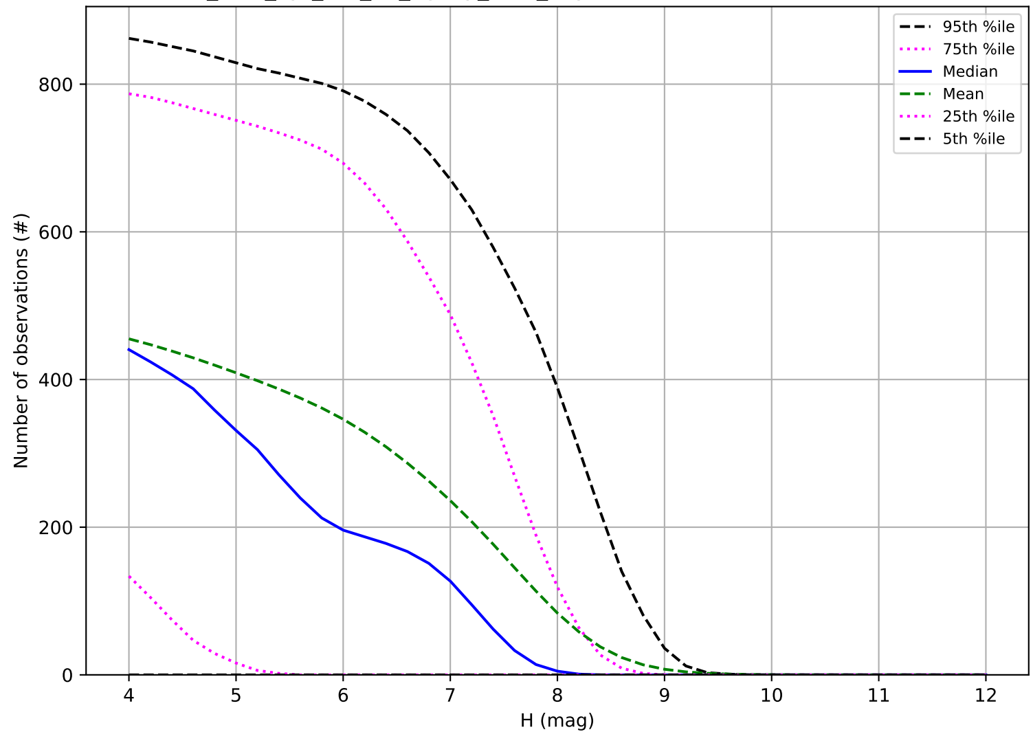
too_elab_2yr_r32_d2_ugrizy_v3.4_10yrs: Number of observations TNO
