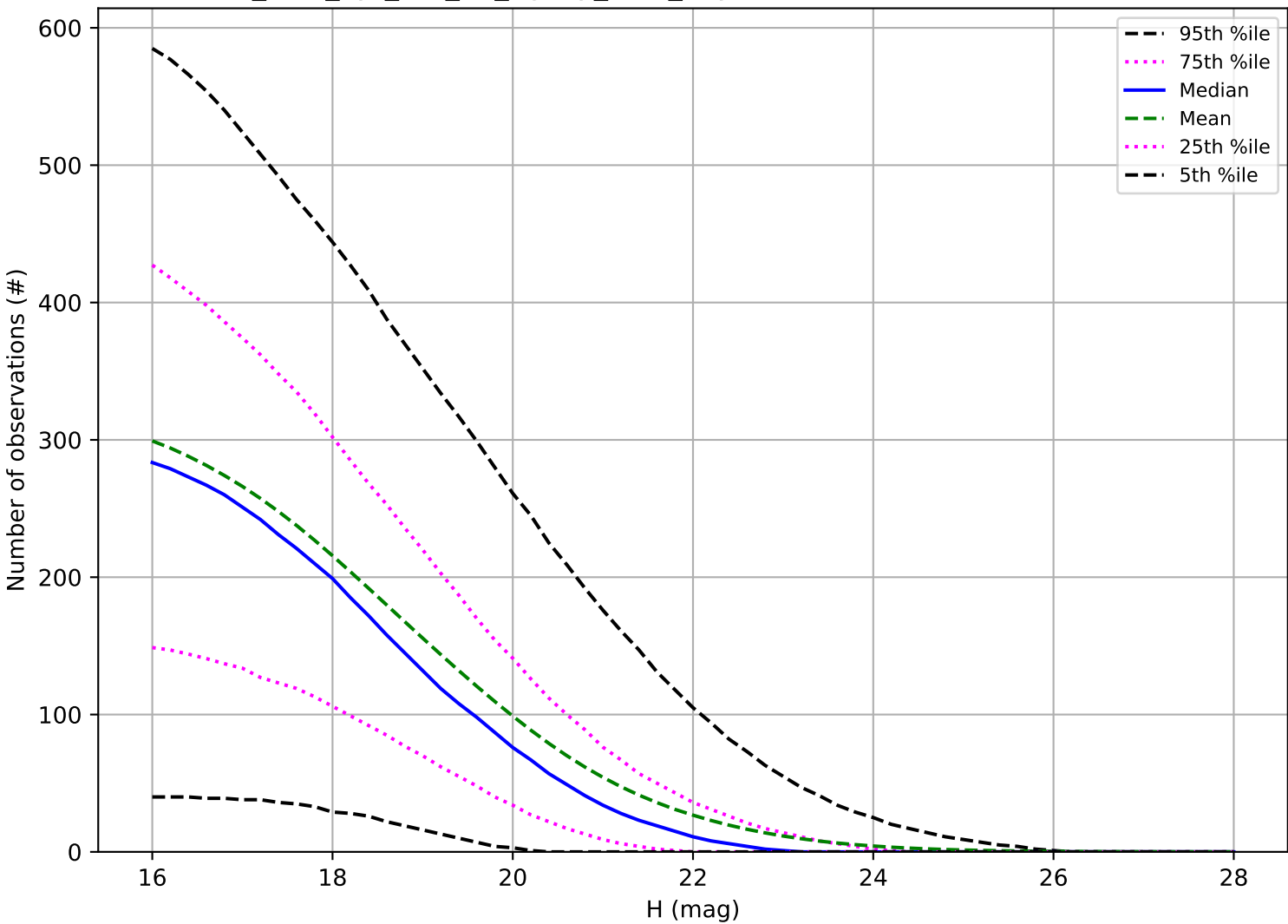
too_elab_2yr_r32_d2_ugrizy_v3.4_10yrs: Number of observations PHA
