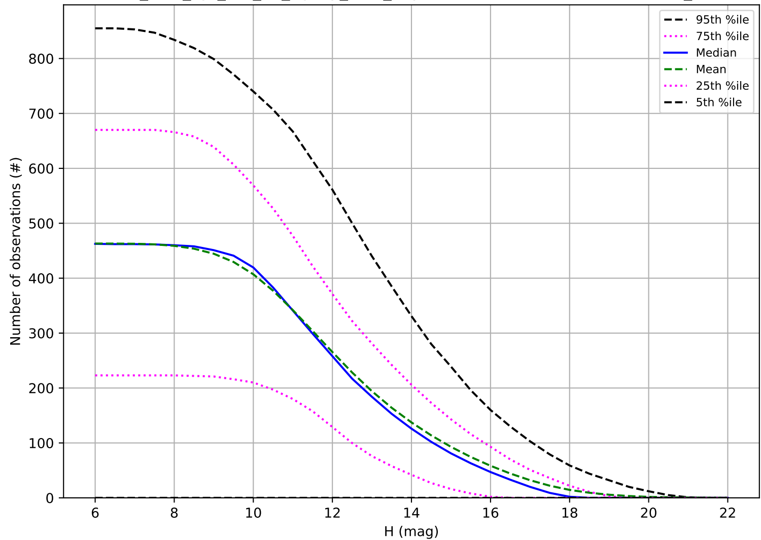
too_elab_2yr_r32_d2_ugrizy_v3.4_10yrs: Number of observations OCC_r5
