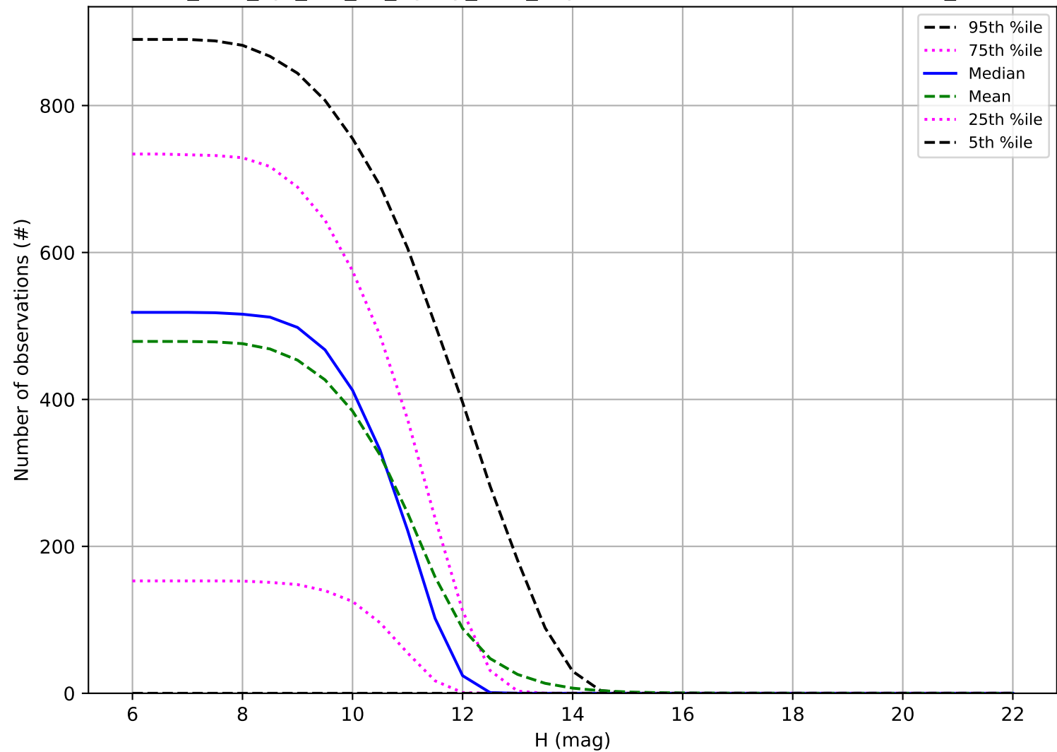
too_elab_2yr_r32_d2_ugrizy_v3.4_10yrs: Number of observations OCC_r20
