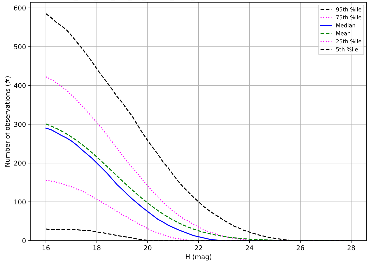
too_elab_2yr_r32_d2_ugrizy_v3.4_10yrs: Number of observations NEO
