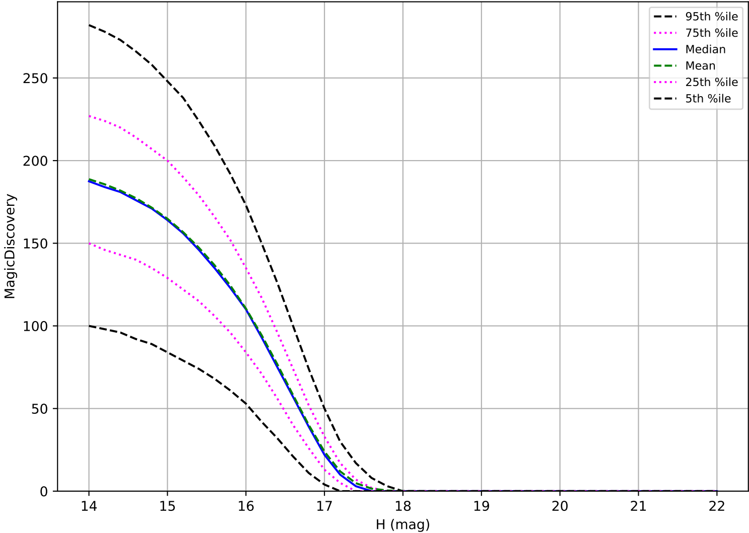
too_elab_2yr_r32_d2_ugrizy_v3.4_10yrs: Trojan 6 detections in 60 nights detection loss
