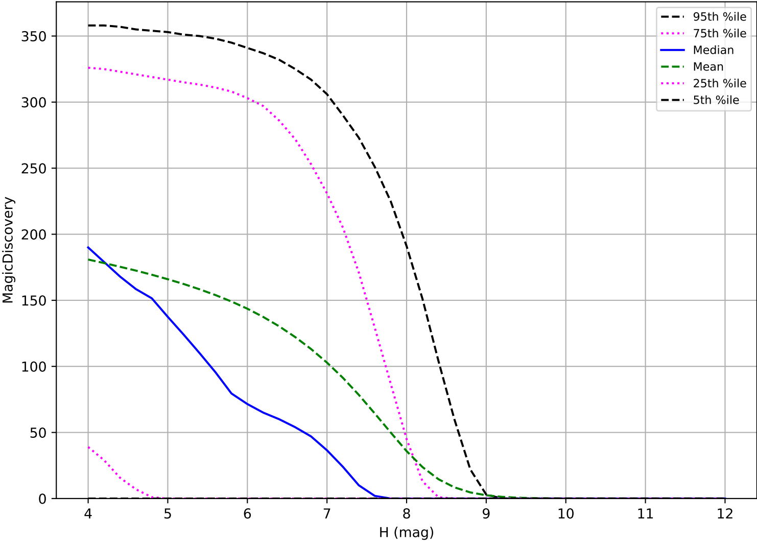
too_elab_2yr_r32_d2_ugrizy_v3.4_10yrs: TNO 6 detections in 60 nights detection loss
