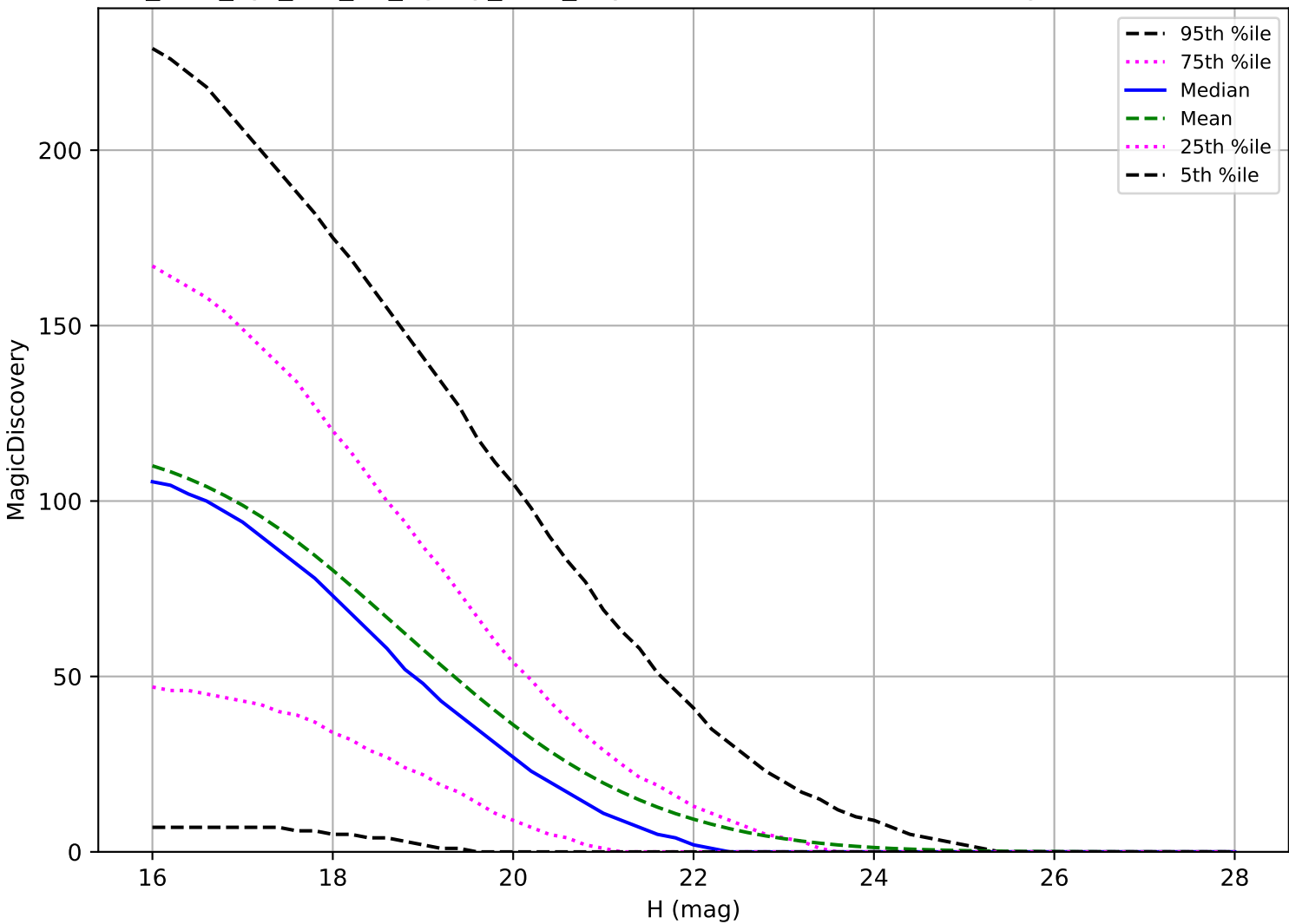
too_elab_2yr_r32_d2_ugrizy_v3.4_10yrs: PHA 6 detections in 60 nights detection loss
