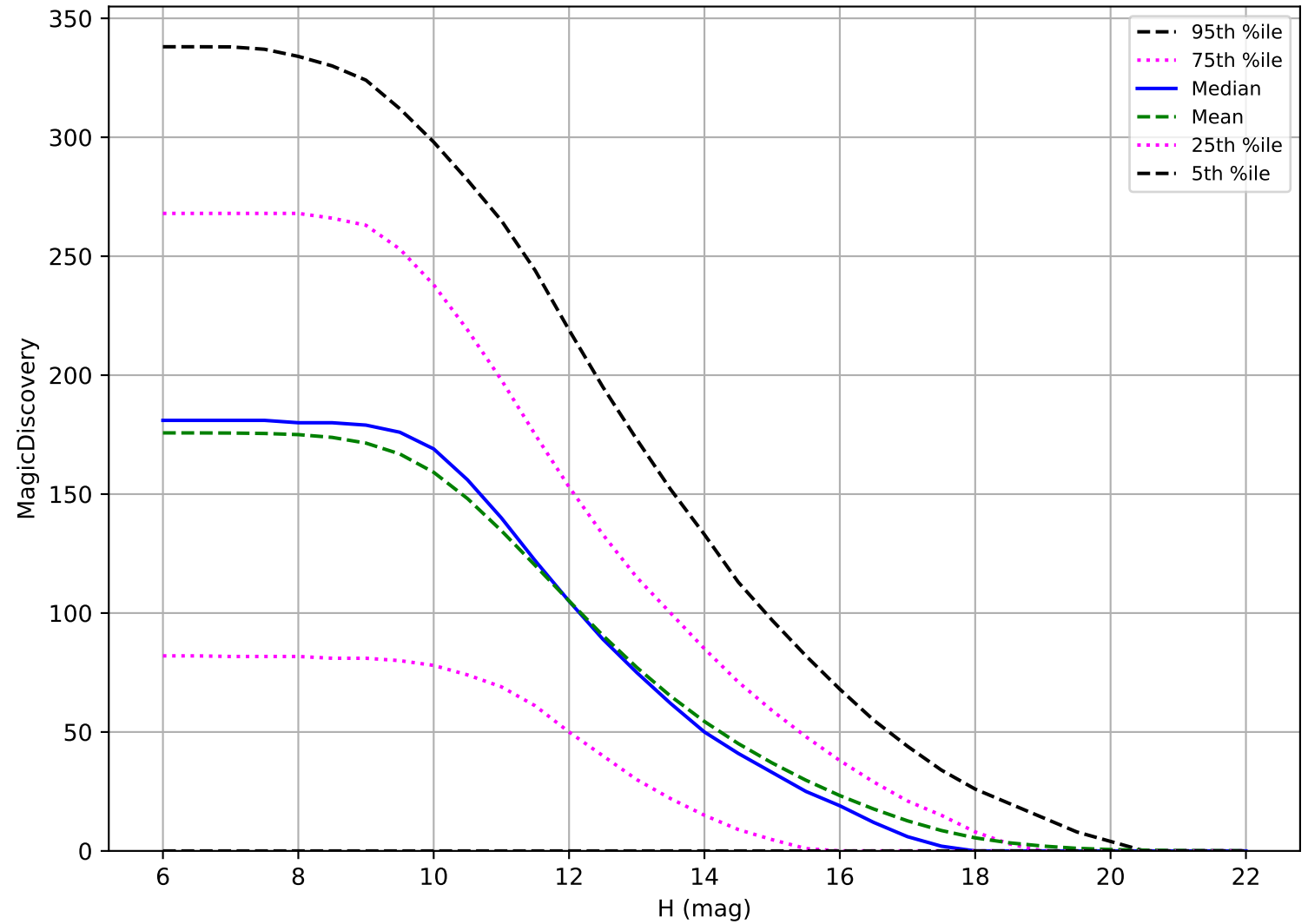
too_elab_2yr_r32_d2_ugrizy_v3.4_10yrs: OCC_r5 6 detections in 60 nights detection loss
