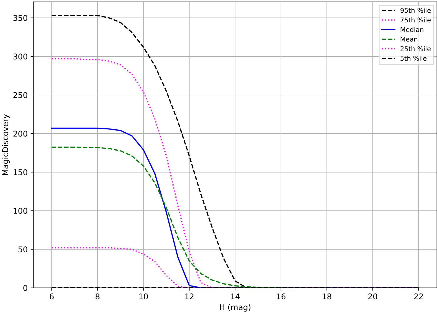
too_elab_2yr_r32_d2_ugrizy_v3.4_10yrs: OCC_r20 6 detections in 60 nights detection loss
