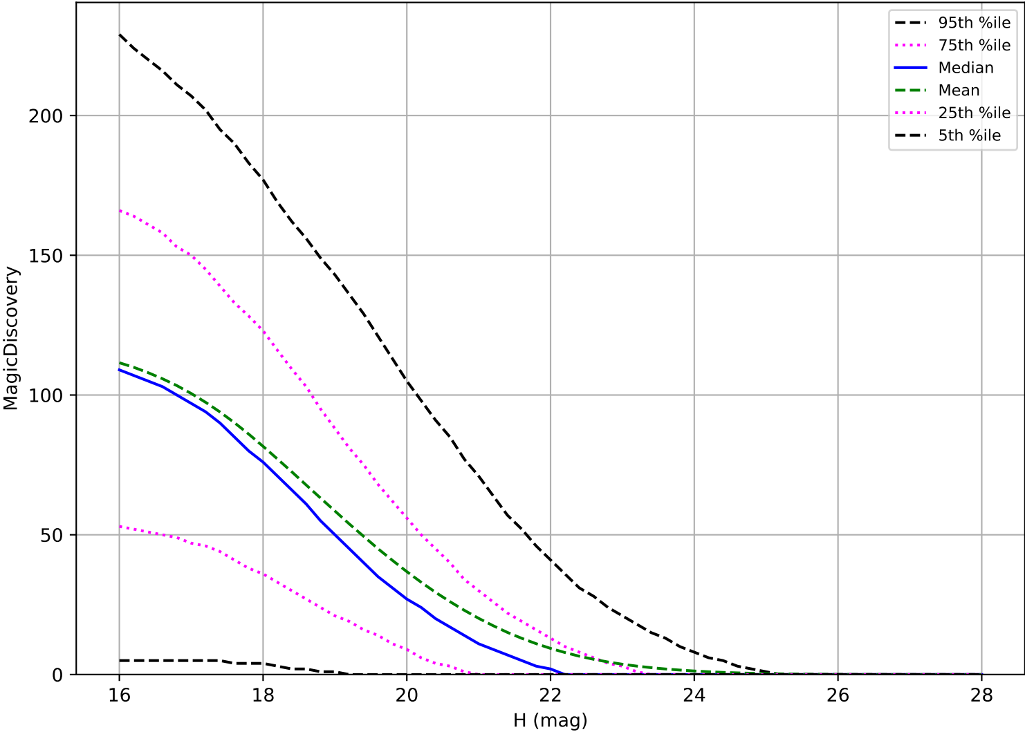
too_elab_2yr_r32_d2_ugrizy_v3.4_10yrs: NEO 6 detections in 60 nights detection loss
