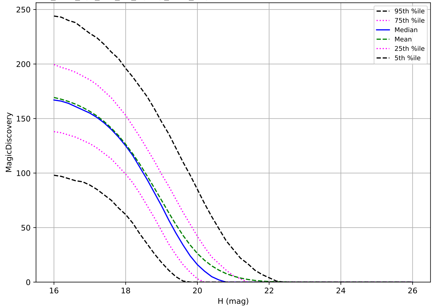
too_elab_2yr_r32_d2_ugrizy_v3.4_10yrs: MBA 6 detections in 60 nights detection loss
