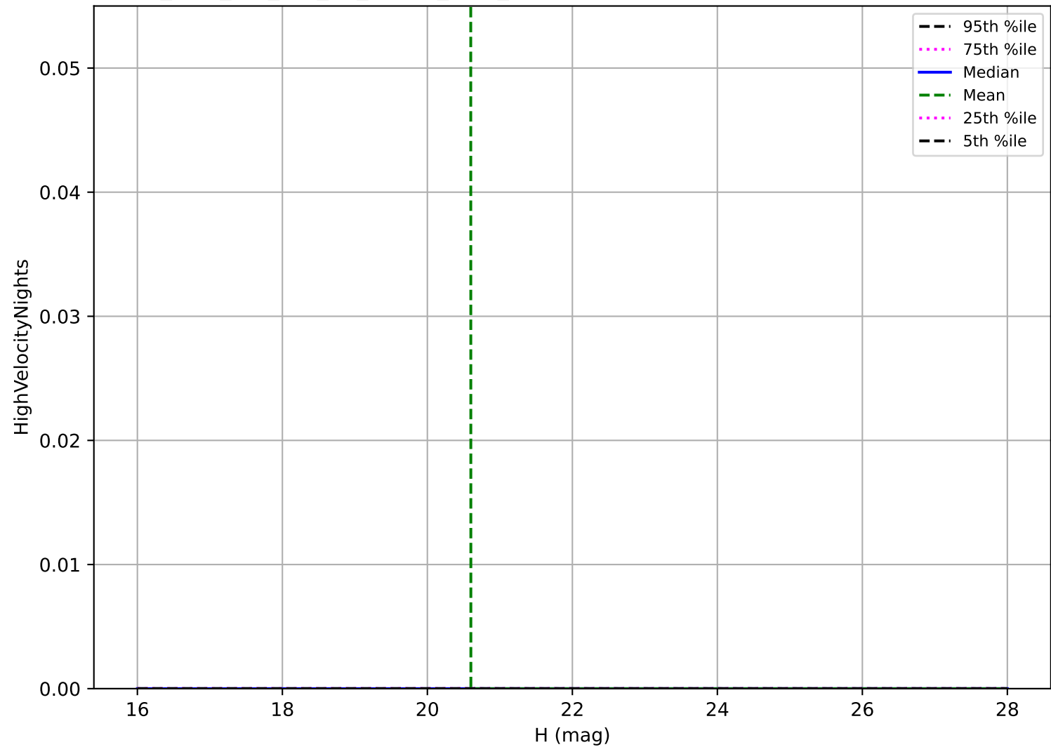
too_elab_2yr_r32_d2_ugrizy_v3.4_10yrs: Vatira High velocity pair detection loss
