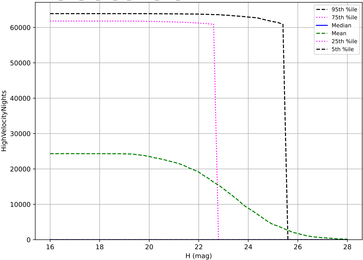
too_elab_2yr_r32_d2_ugrizy_v3.4_10yrs: PHA High velocity pair detection loss
