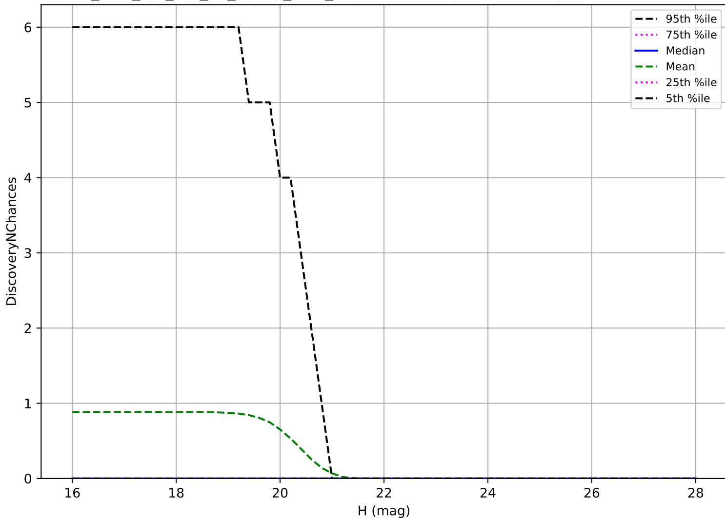
too_elab_2yr_r32_d2_ugrizy_v3.4_10yrs: Vatira 3 pairs in 15 nights detection loss
