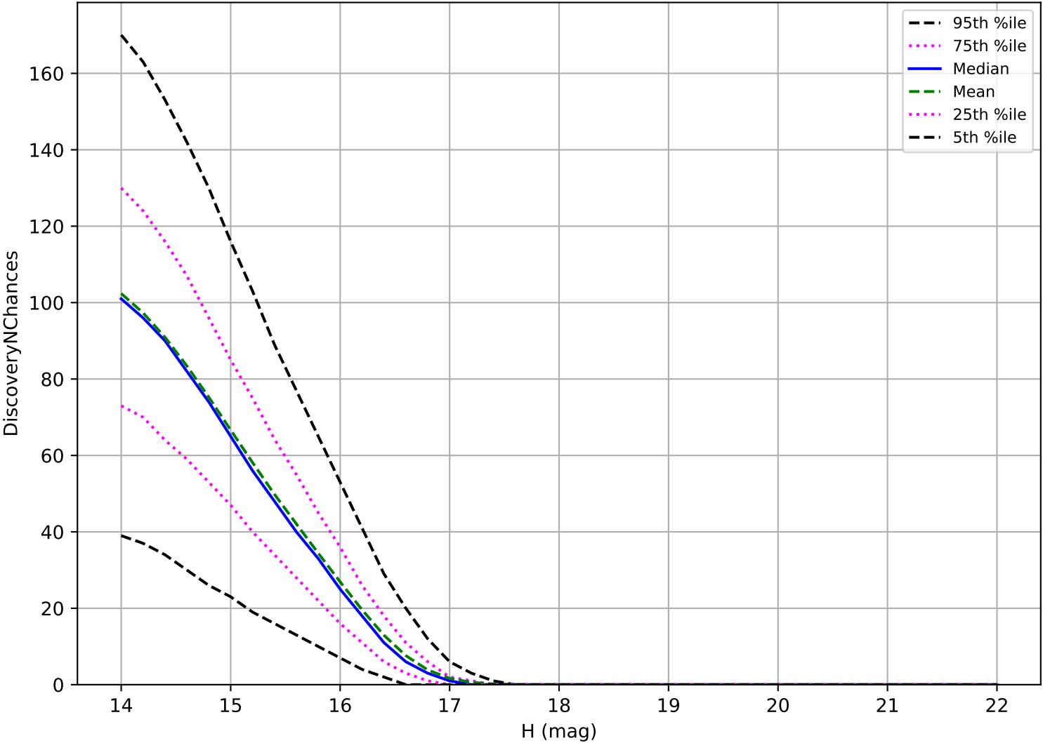
too_elab_2yr_r32_d2_ugrizy_v3.4_10yrs: Trojan 3 pairs in 15 nights detection loss
