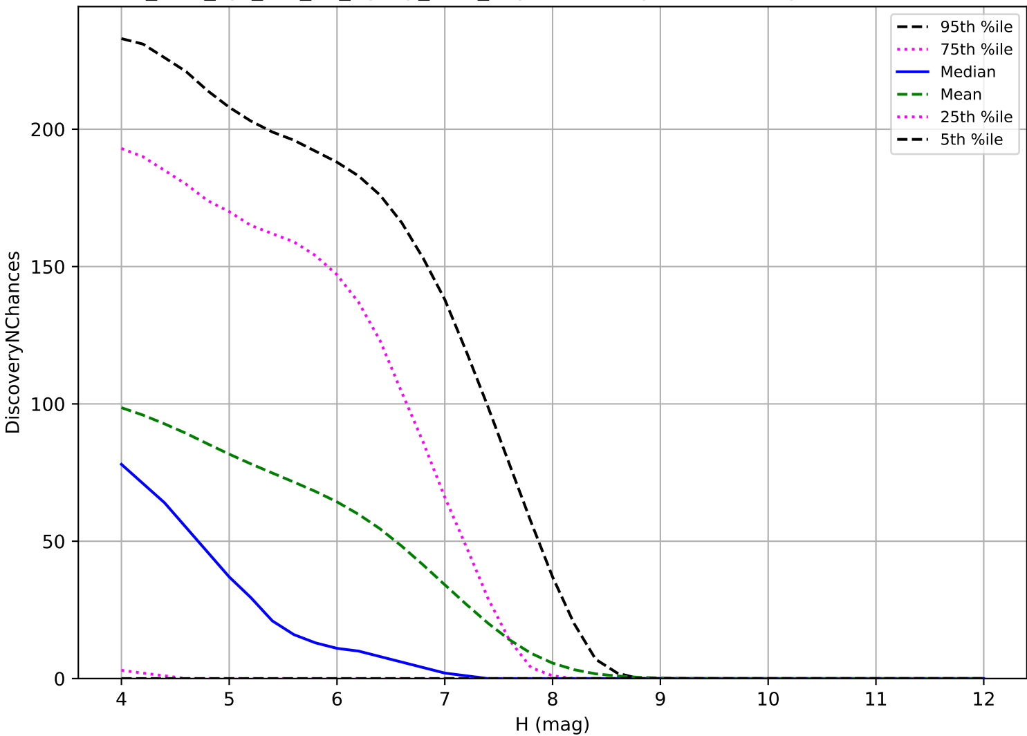
too_elab_2yr_r32_d2_ugrizy_v3.4_10yrs: TNO 3 pairs in 15 nights detection loss
